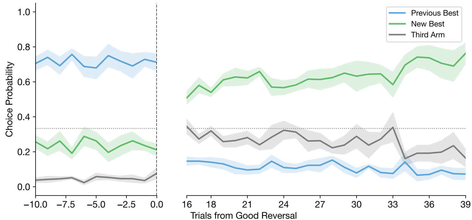
Good Reversal-Aligned Choices (mean \pm se across subjects | n=6 subjects, n=241 reversals) (Skipping first 15 trials post-reversal)
